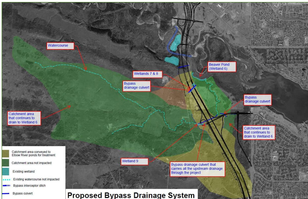
Figure 17: bypass drainage for Spring Brook (northern culvert) and Ravine Creek (southern culvert) intended to maintain surface flow across the Transportation Utility Corridor into the Beaver Pond ( Sept. 201, courtesy of KGL – construction company for the SWCRR )
